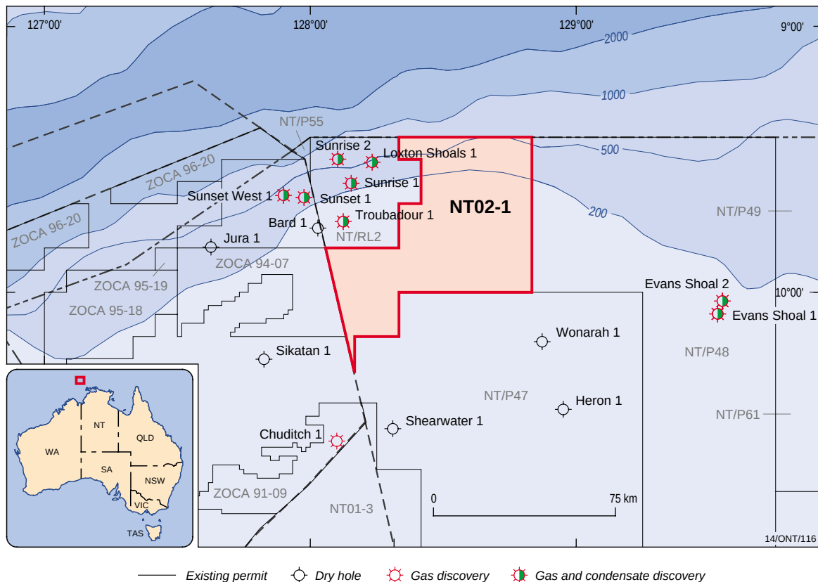
Figure 1. Location map showing release area, Sahul Platform, northern Bonaparte Basin.
